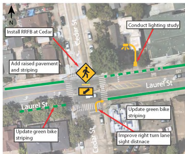
Figure 28. Laurel Street Corridor (from Washington Street to Front Street) Countermeasure Opportunities
