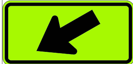
DETAIL A7 W16-7P(L) SIGN (30"x18")
